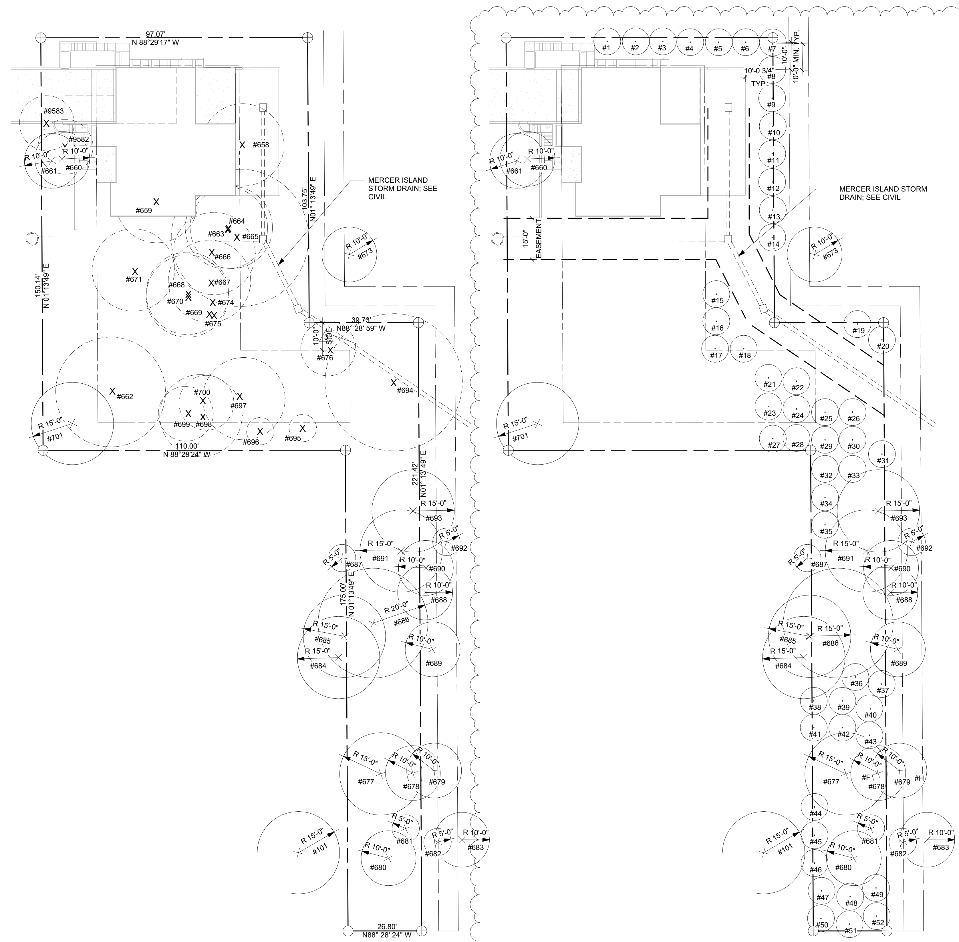
TREE RETENTION DIAGRAM 1" = 20'-0" 1 PROPOSED TREE DIAGRAM 1" = 20'-0" 2
